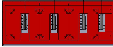
SECTION B-B SCALE 1 : 20 INSULATED GLASTIC BARRIER
